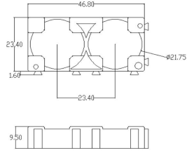
21700-2P Battery Holder Diameter: 21.7mm Distance: 23.4mm Material:ABS
