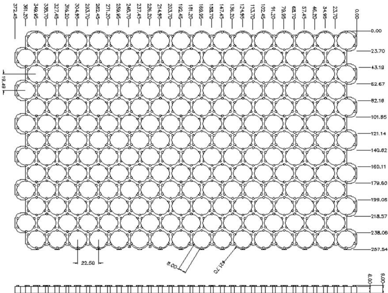
21700 Battery holder, cell spacing 22.5mm, diameter 21.3/21.7mm, non-assembly type. Available size:1x1-13x16
