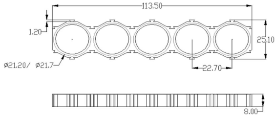
21700-5P Honeycomb Battery Holder Diameter: 21.2mm/21.7mm Distance: 22.7mm Material:ABS
