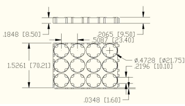
21700-3x4 Battery Holder Diameter: 21.7mm Distance: 23.4mm Material:ABS
