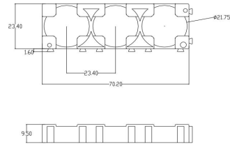
21700-3P Battery Holder Diameter: 21.7mm Distance: 23.4mm Material:ABS
