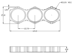
21700-3P Honeycomb Battery Holder Diameter: 21.2mm/21.7mm Distance: 22.7mm Material:ABS
