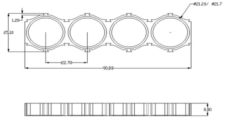
21700-4P Honeycomb Battery Holder Diameter: 21.2mm/21.7mm Distance: 22.7mm Material:ABS
