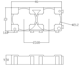
21700-2P Battery Holder Diameter: 21.2mm Distance: 23mm Material:ABS/ ABS+PC
