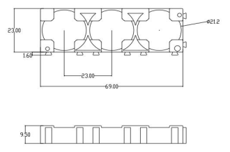
21700-3P Battery Holder Diameter: 21.2mm Distance: 23mm Material:ABS/ ABS+PC
