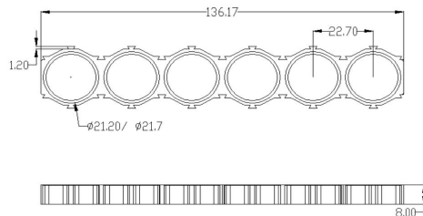
21700-6P Honeycomb Battery Holder Diameter: 21.2mm/21.7mm Distance: 22.7mm Material:ABS
