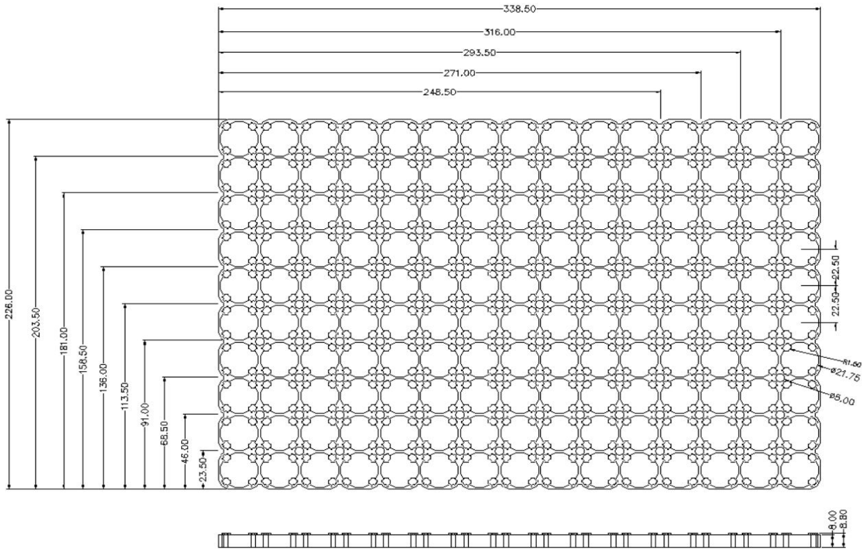
21700 Battery holder, cell spacing 22.5mm, diameter 21.3/21.7mm, non-assembly type. Available size:1x1-13x16
